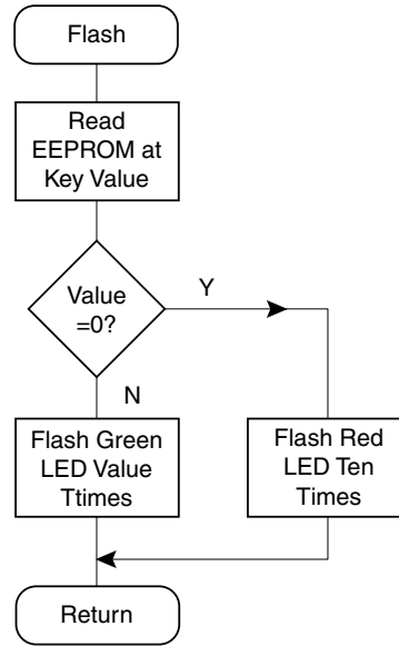
Figure 3. Flowchart for Reset and Main Routine
