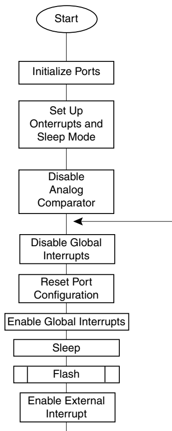
Figure 2. Flowchart for “Flash” Function
