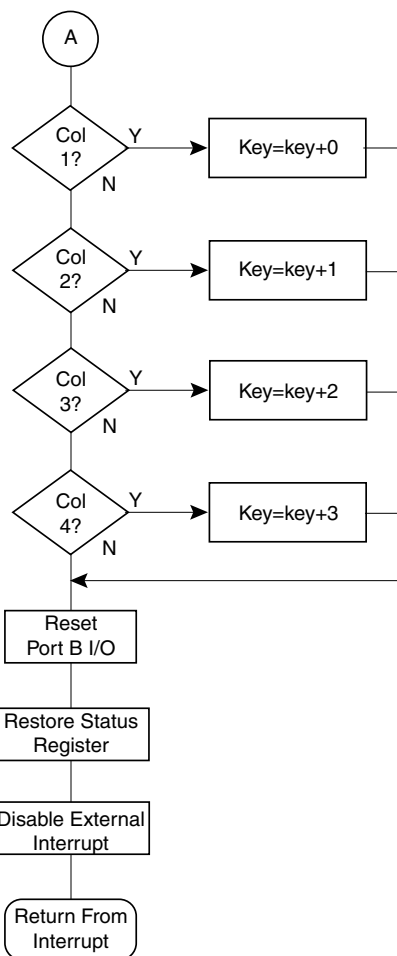
Figure 6. Flowchart for Interrupt Service Routine Continued
