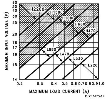
FIGURE 5. LM2575(HV)-12
