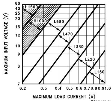
FIGURE 4. LM2575(HV)-5.0
