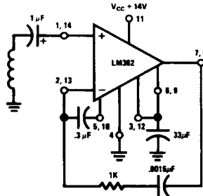
Phono Preamp (RIAA Equalization)
