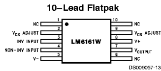
See NS Package Number W10A
