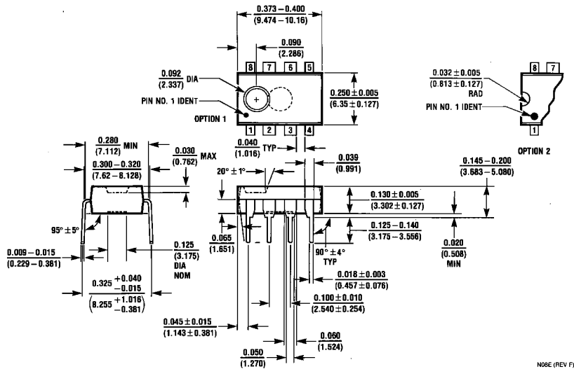
Molded Dual-In-Line Package (N) Order Number LM6261N or LM6361N NS Package Number N08E
