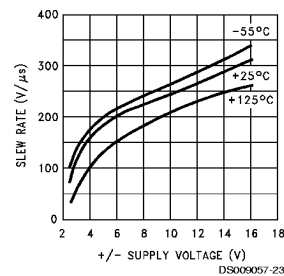
Slew Rate
