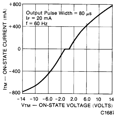
Fig. 2. On-State Characteristics
