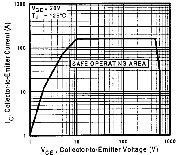
Fig. 12 - Turn-Off SOA
