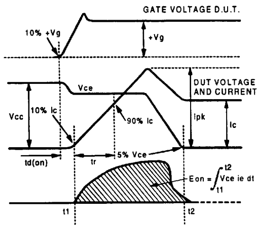
Fig. 18c - Test Waveforms for Circuit of Fig. 18a, Defining E_{on} , t_d(\text{on}) , t_r
