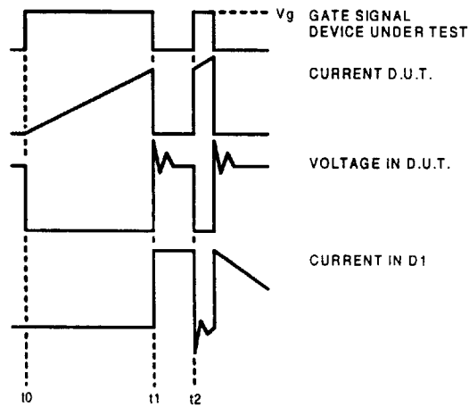
Figure 18e. Macro Waveforms for Figure 18a's Test Circuit
