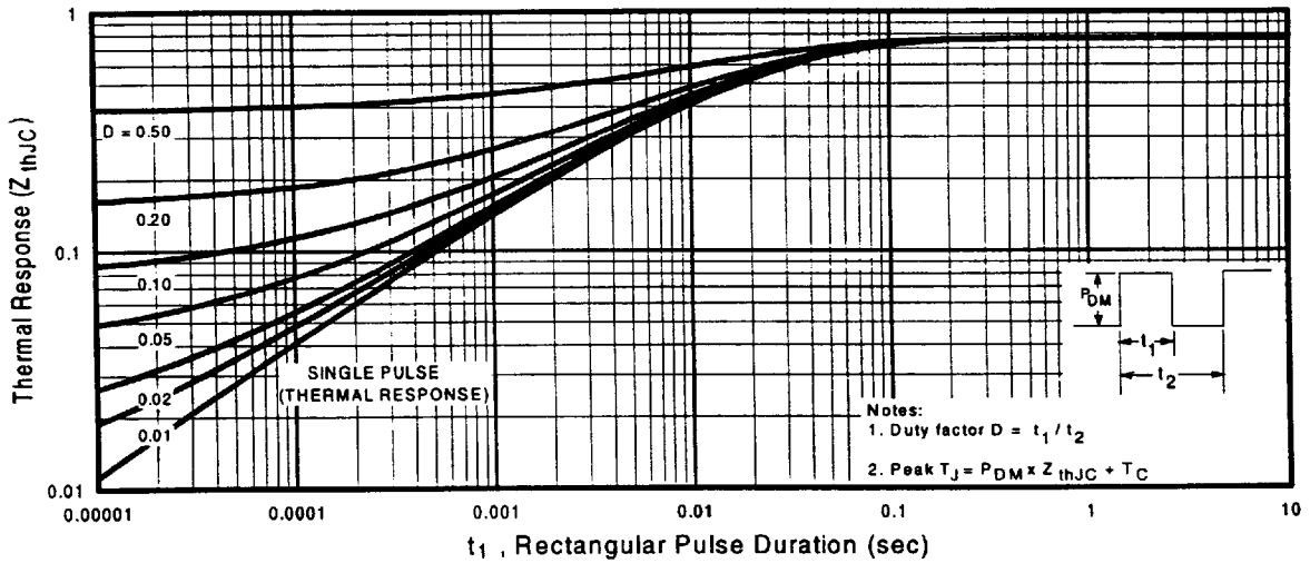
Fig. 6 - Maximum IGBT Effective Transient Thermal Impedance, Junction-to-Case
