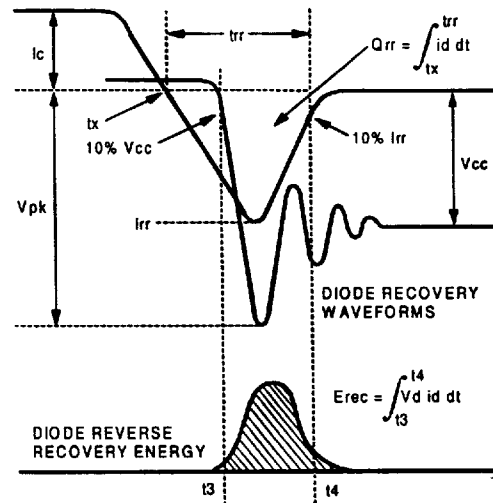
Fig. 18d - Test Waveforms for Circuit of Fig. 18a, Defining E_{rec} , t_{rr} , Q_{rr} , I_{rr}
