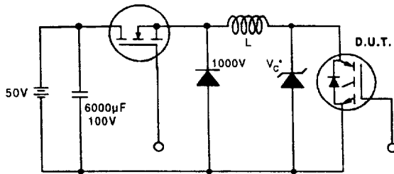
Figure 19. Clamped Inductive Load Test Circuit
