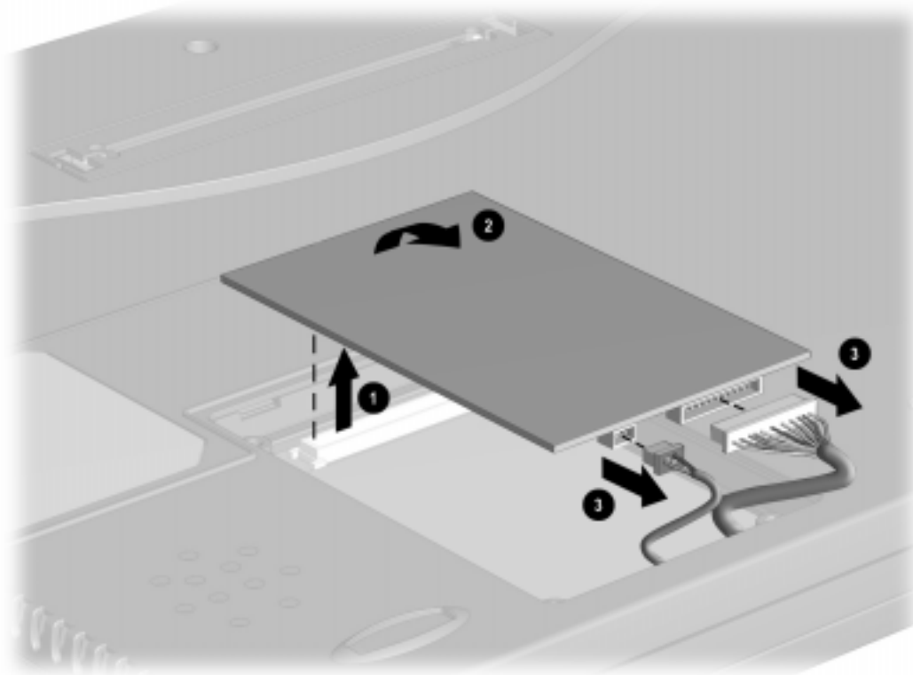
Figure 5-12. Removing the Modem or Modem/NIC Card
