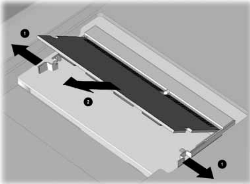
Figure 5-16. Removing the Memory Board
