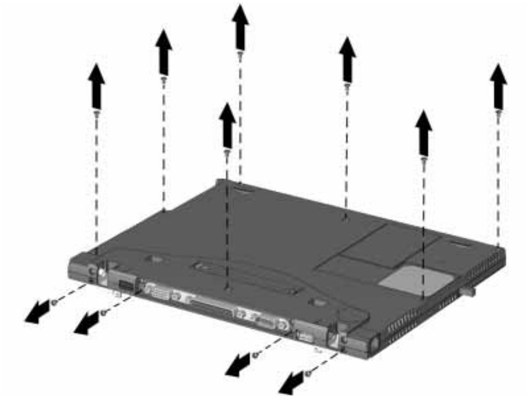
Figure 5-21. Removing the Top Cover Screws
